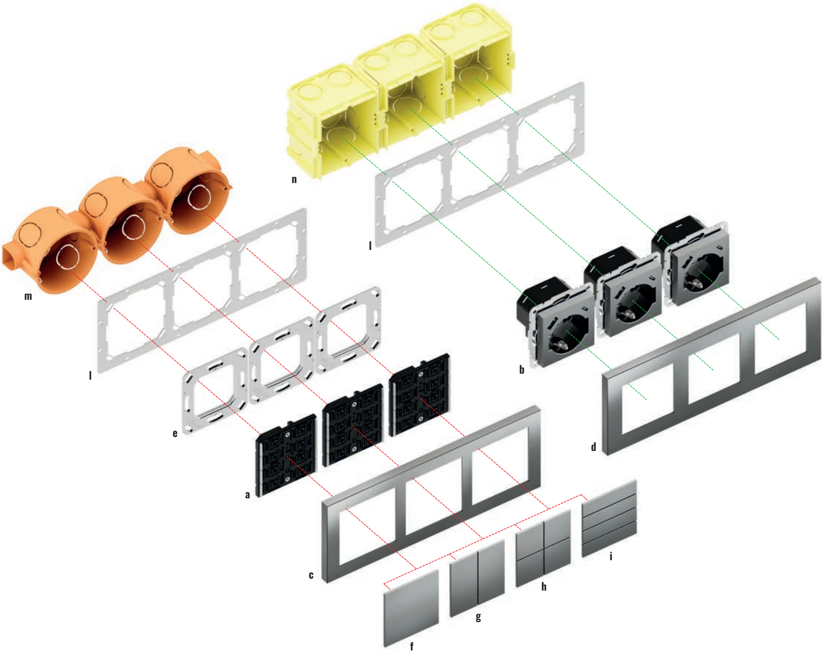
Triple installation with centre distance 71 mm (71 series)
